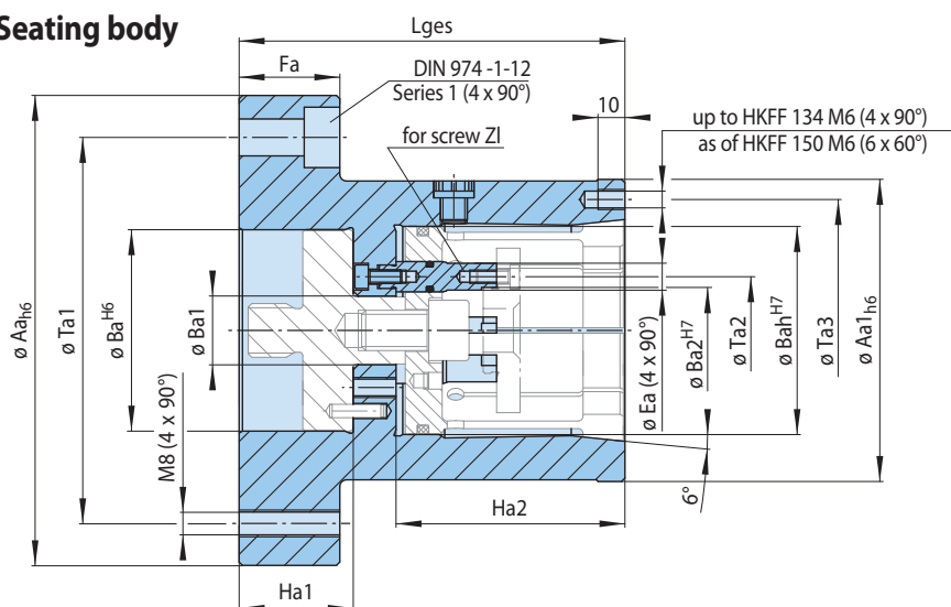
for sizes HKFF 66 and HKFF 76
