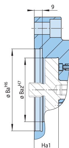
for sizes HKFF 86 to HKFF 225
